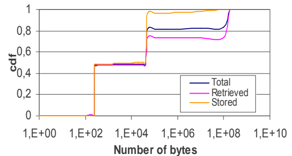
Figure 8: Empirical cdf's of the grid-ftp transfer sizes
